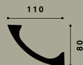
WT3 WALLSTYL® 80 x 110 x 2000 mm
